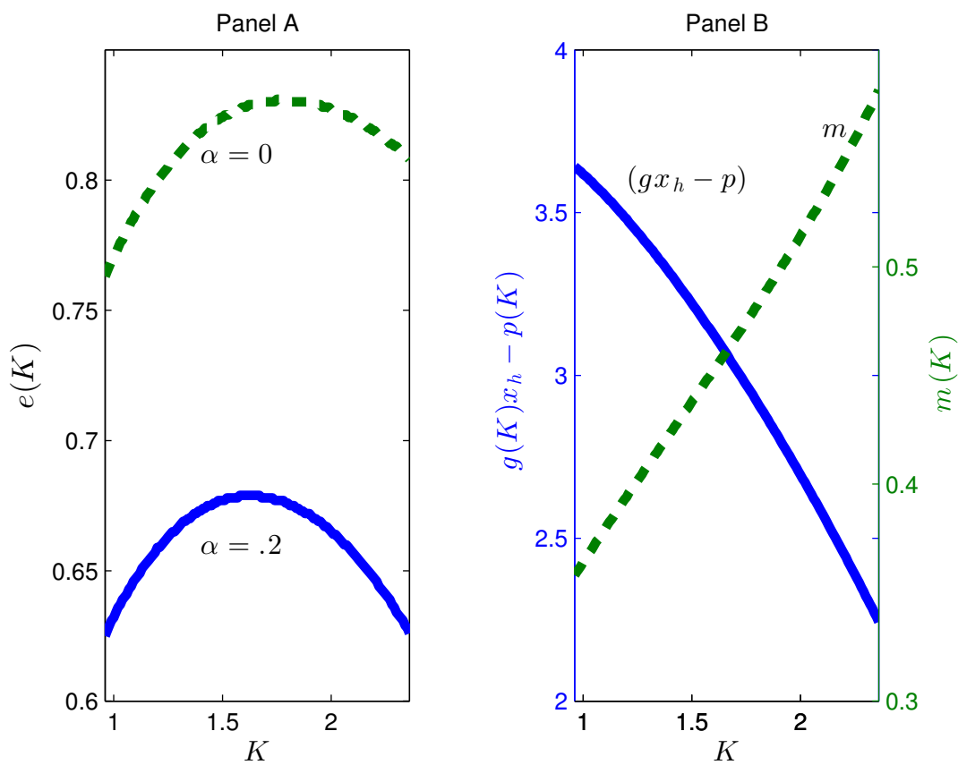
Figure 3: Panel A: Origination effort e , as a function of capital, K , for the cases \alpha = 0 (dashed line, in green) and \alpha = .2 (continuous line, in blue). Panel B: x_h p , as a function of capital K (continuous line, in blue, left axis) and matching probability m as a function of capital, K , (dashed line, in green, right axis). In this example, \psi(e) = \theta \frac{e^2}{2} with \theta = .25 . In addition, \kappa = .15 , \eta = .5 , M = .75 and x_h = 5 .
